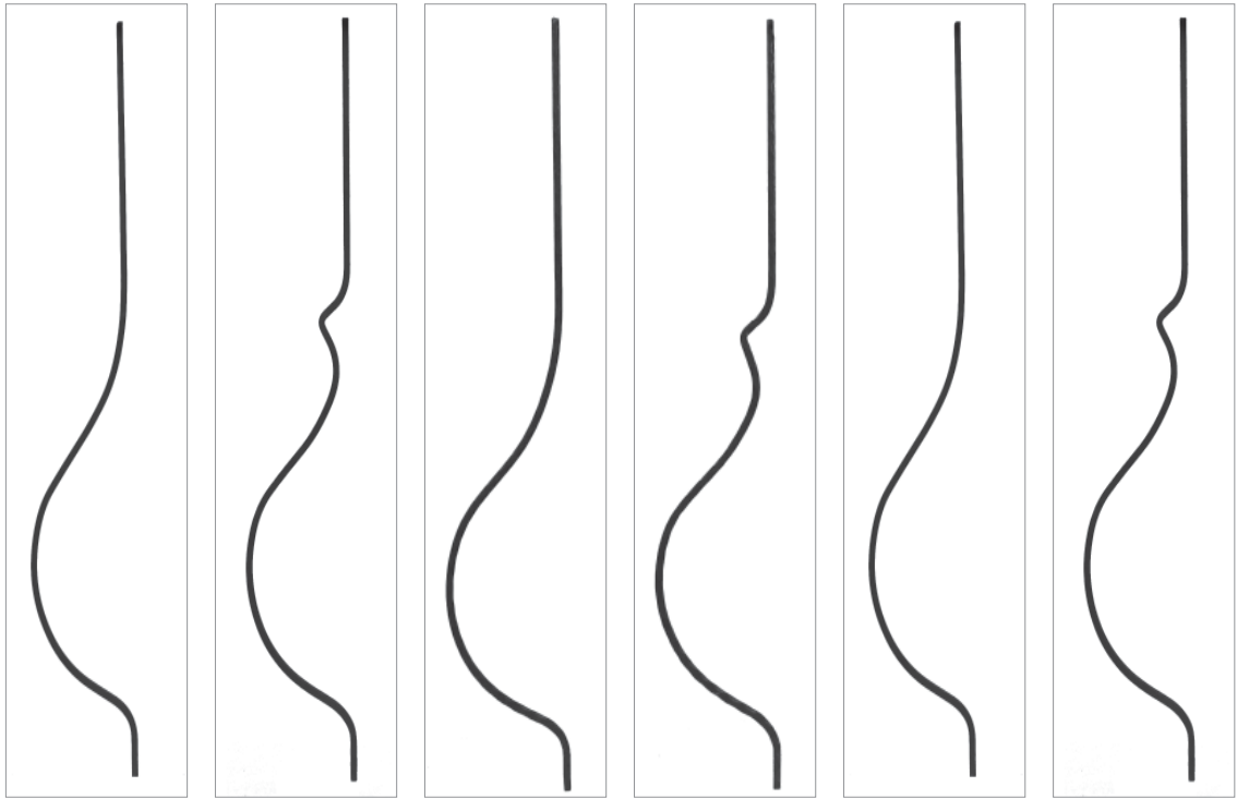
BOW1 BOW2 BOW3 BOW4 BOW5 BOW6 12x12mm 12x12mm 12x12mm 12x12mm 16x16mm 16x16mm PLAIN BAR PLAIN BAR HAM BAR HAM BAR PLAIN BAR PLAIN BAR
