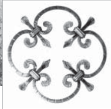
RZ8 250mm DIA 8x8mm SQ BAR
