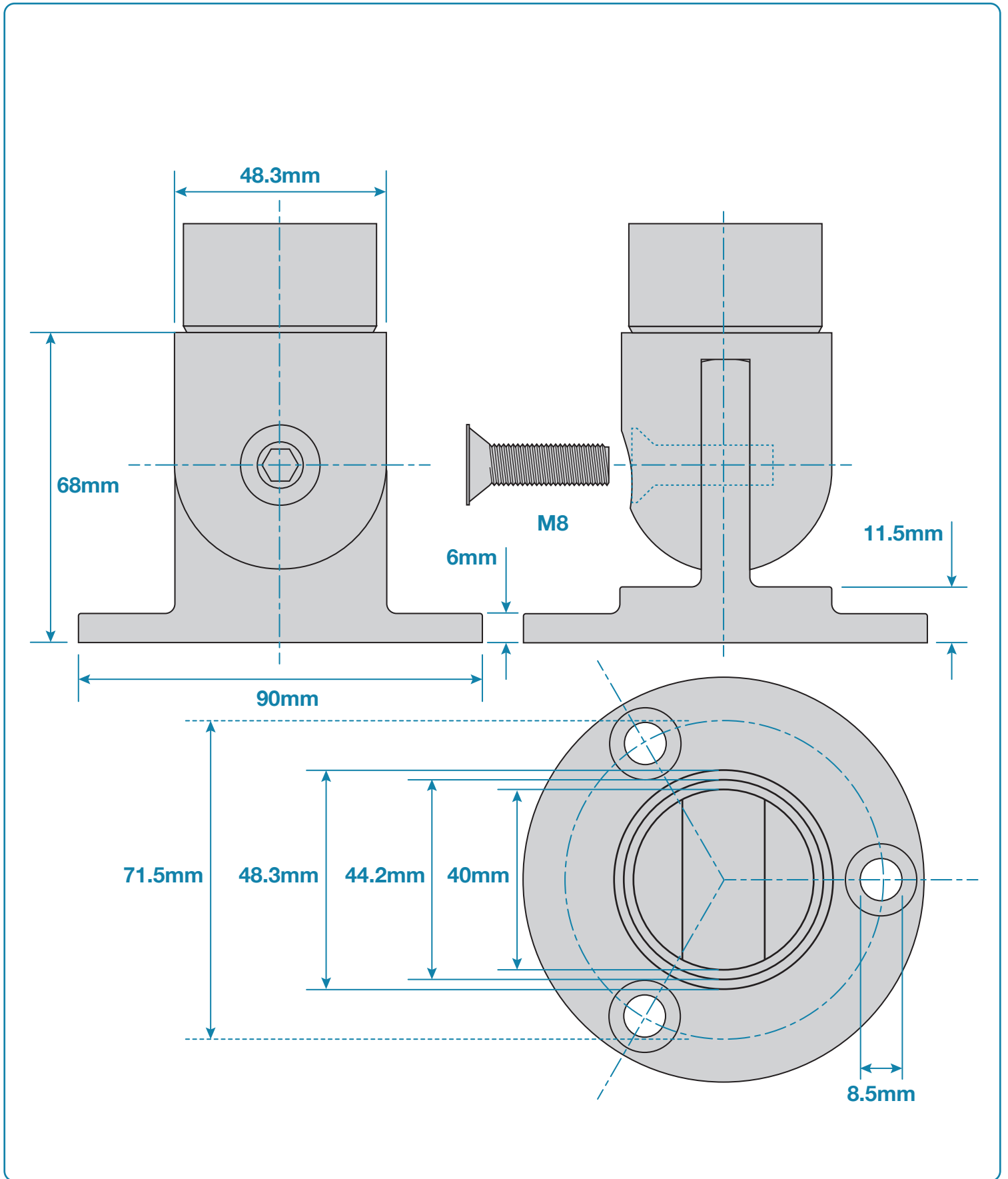
Stainless Steel 304 Adjustable Wall Bracket To Suit 48.3 x 2mm Tube
