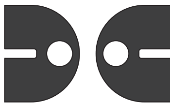
Rubber gaskets to fit 4mm and 6mm glass
