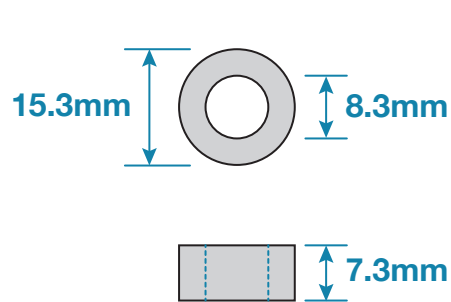
Nylon spacer
