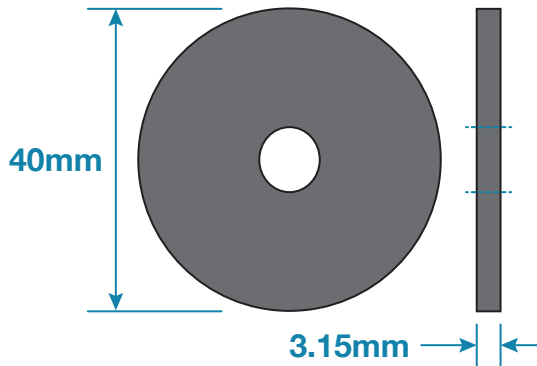
Rubber disc
