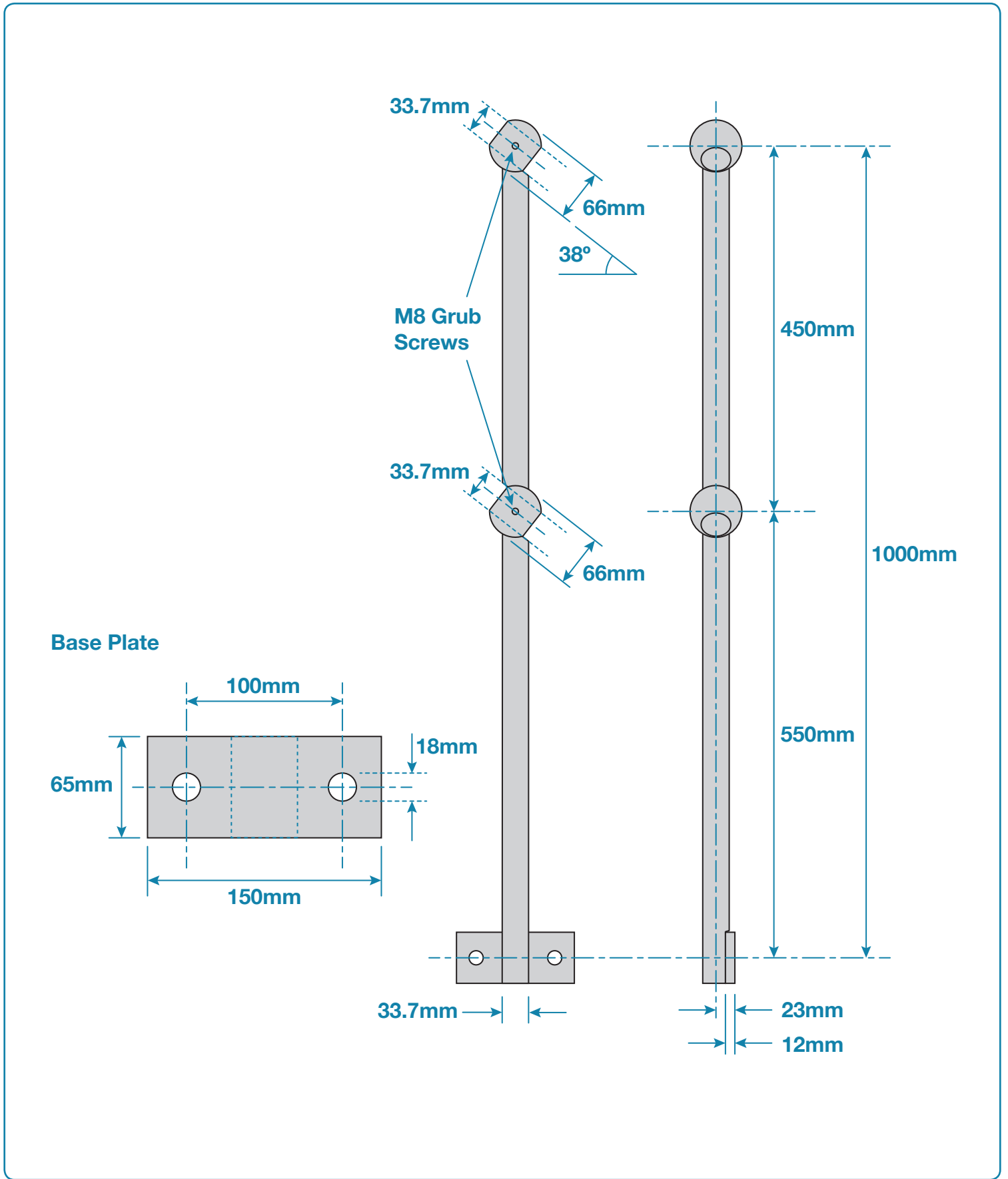
Galvanised Handrail Standard With Rake Side Palm, Right To Suit Tube 33.7mm
