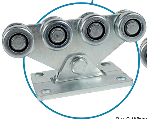
2 x 8 Wheel Carriages, these run inside the guide track and should be bolted down to concrete foundation
