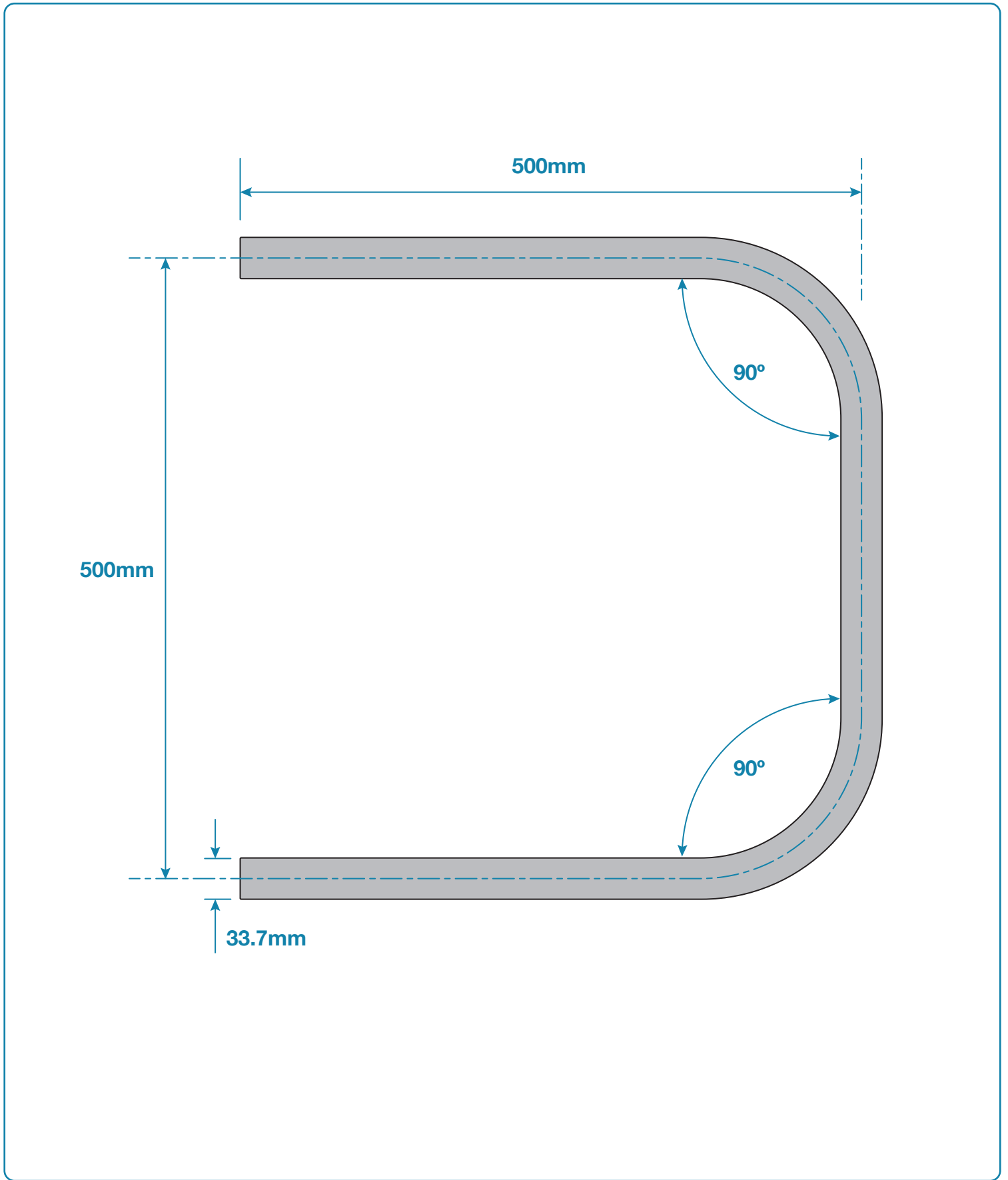
Galvanised Modular Rail Platform Return Bend 33.7mm Tube
