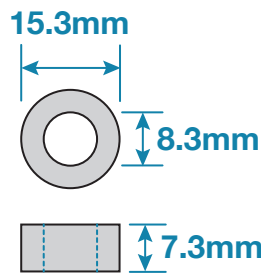
Nylon spacer
